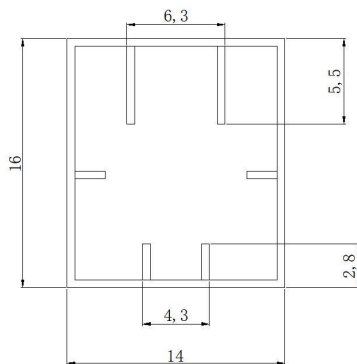
Fig.8 Section schematic diagram
