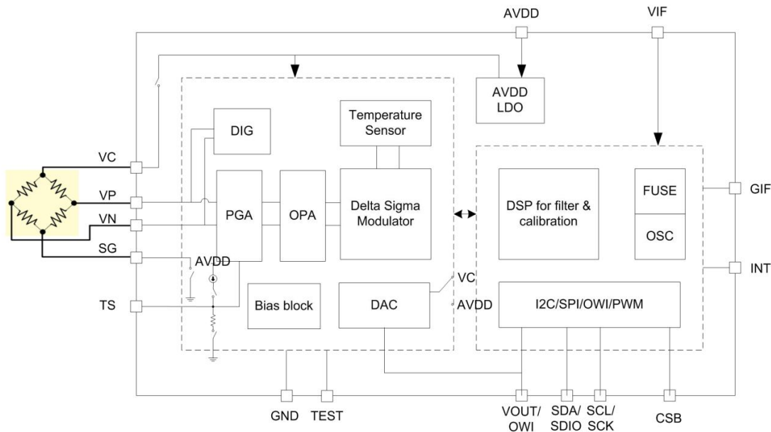
Fig.1 Block Diagram
