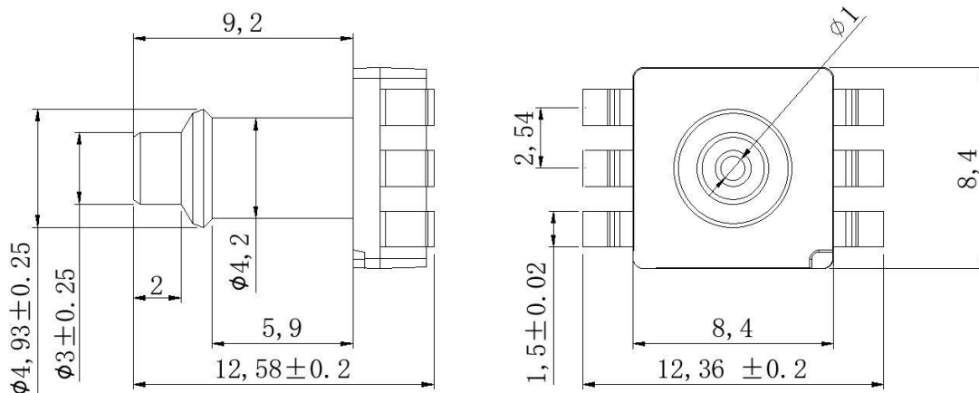
Fig.6 Sensor Dimensions
