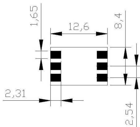
Fig.7 Recommended Footprint
