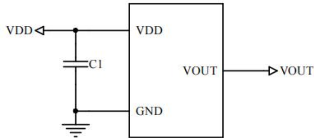
Fig.5 Application circuit
