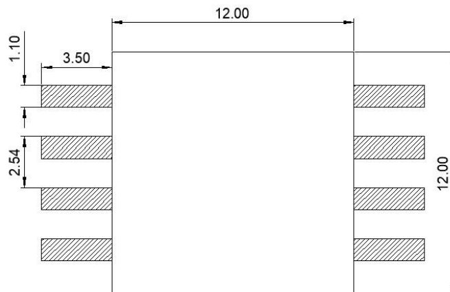
Fig.7 Recommended Footprint
