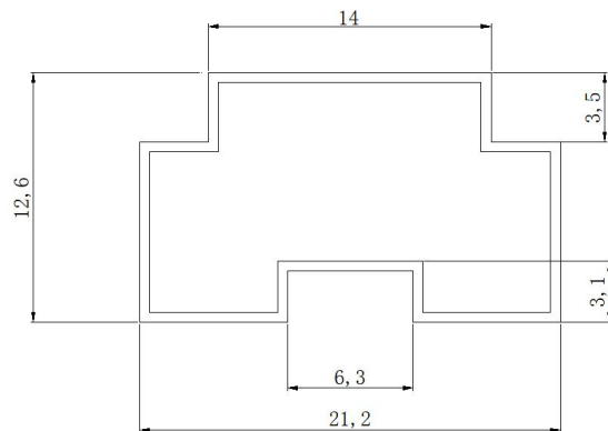
Fig.8 Section schematic diagram
