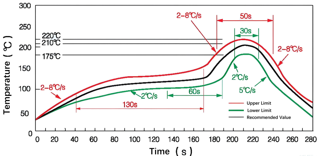
Fig.8 Remelting temperature setting conditions
