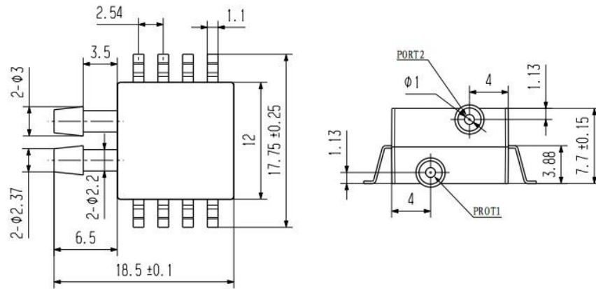
Fig.6 Sensor Dimensions
