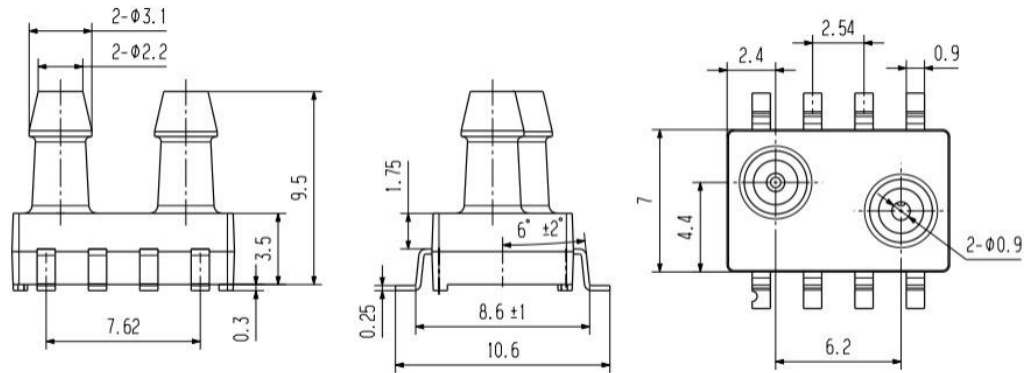
Fig.8 Product dimensions
