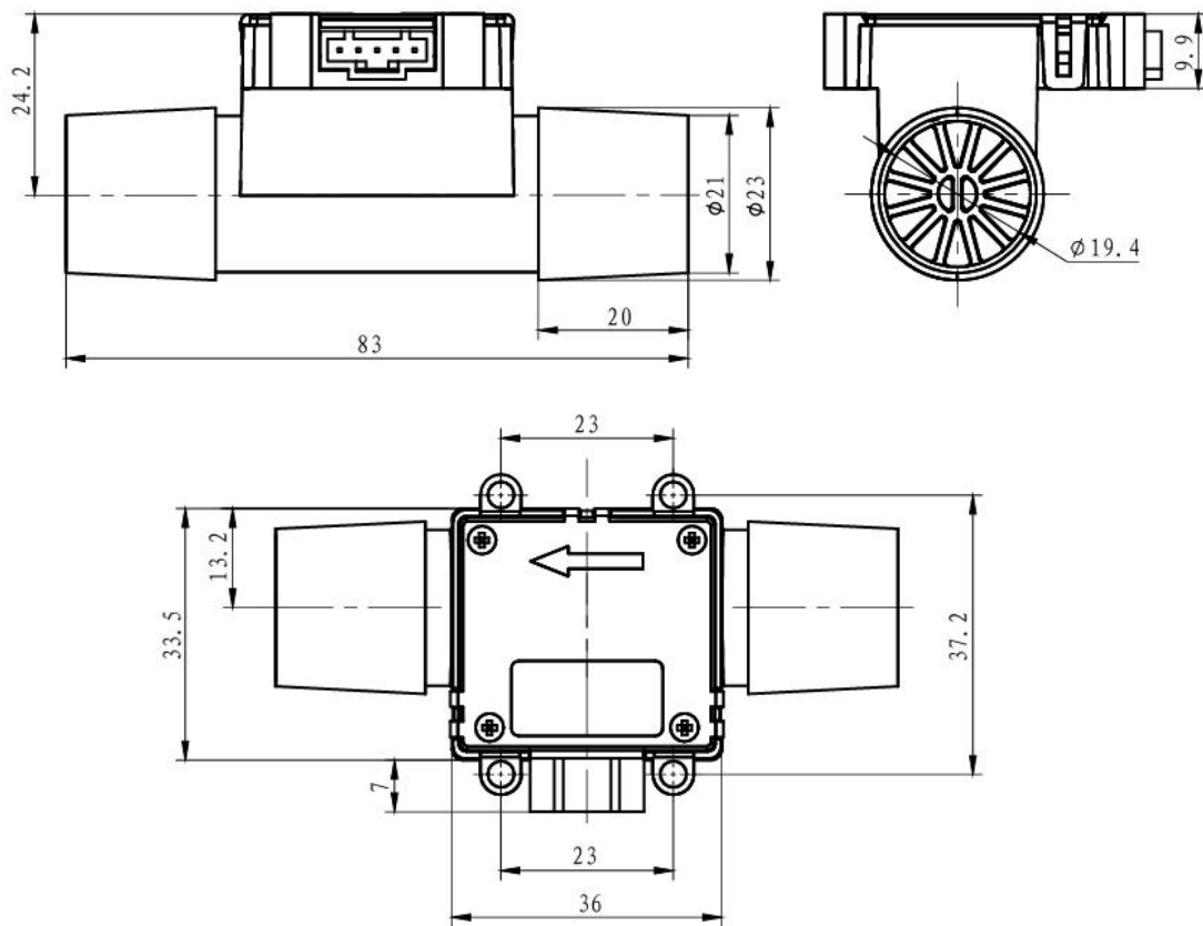
Fig.1 Sensor dimensions
